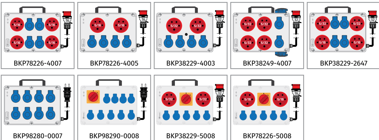
Handled Cabled Powerbox 210x300x90mm
